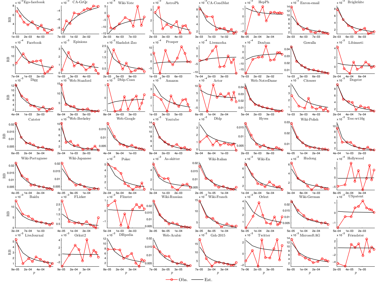
Figure 3: The observed vs. estimated RB of \hat{C} . The results were obtained over 5 \times 10^4 independent runs for all graphs except for the large graphs in the last row with 10^4 . The estimated RBs are obtained using Eq. 16.
